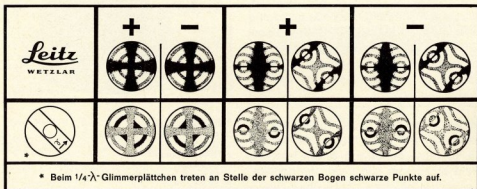
Fig. 9 Table for the determination of the character of birefringence
