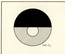
Fig. 12 Correct position of the aperture diaphragm and useful aperture limitation (image with the Bertrand lens turned in or the eyepiece removed and Berek prism in the beam)
